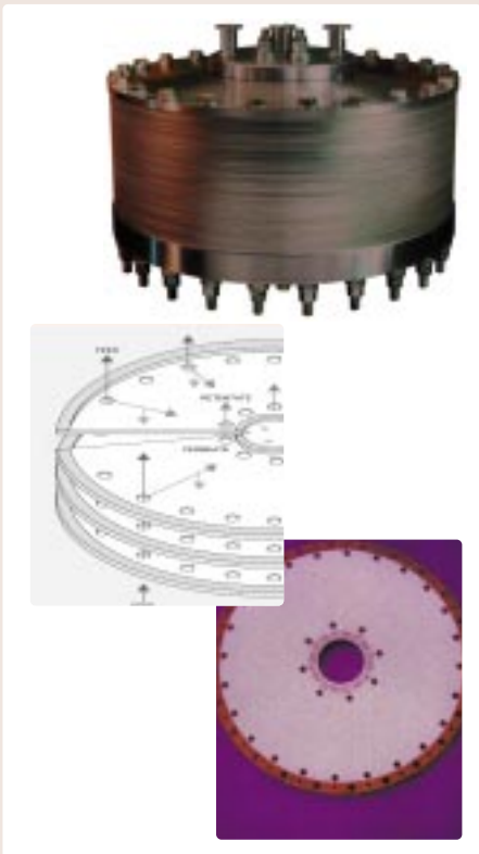
Figure 8: Diagram and photo showing the 40m 2 crossflow filter head of the Pallsep VMF – supplied by Pall Europe Ltd.
