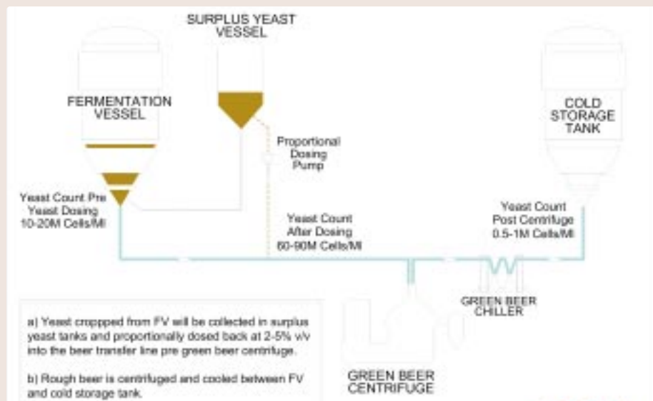
Figure 13: Process diagram of a yeast dose-back pre-centrifuge process – Diagram supplied by CAL Systems Ltd.
